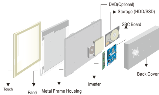
Mechanical design
